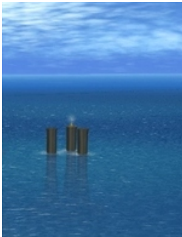
Figure 5. Illustrations of options for leaving the concrete substructure in situ, entirely with navigation lights (left) and cut down to the storage cells. Examples from Frigg cessation plan where the illustration to the left represents the approved solution for Frigg. Source: Total E&P Norge AS.
